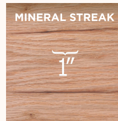
MINERAL STREAK
